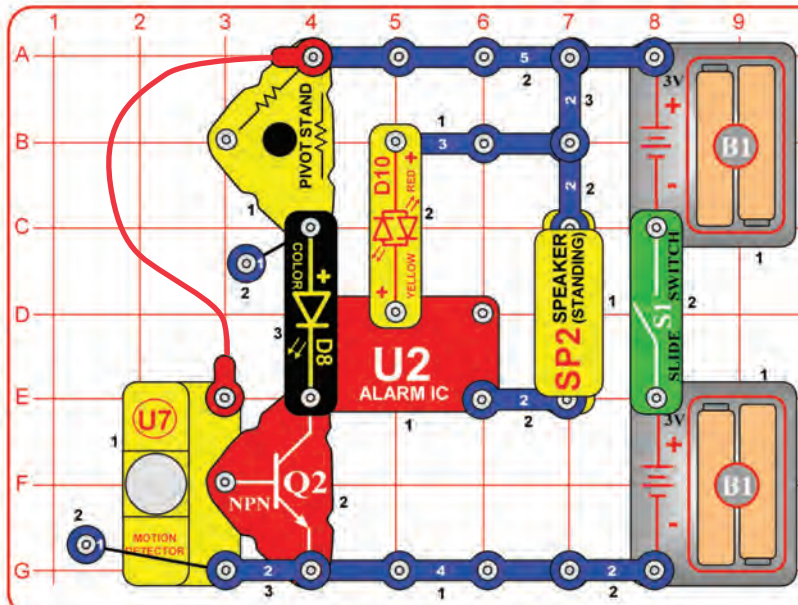
Mount circuit on the blue stand and face across a room.
