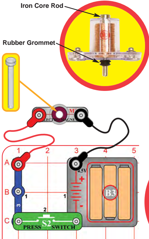
Iron Core Rod
